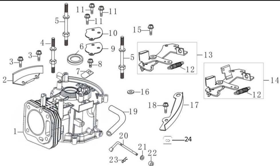
曲轴箱 (CRANK CASE)
